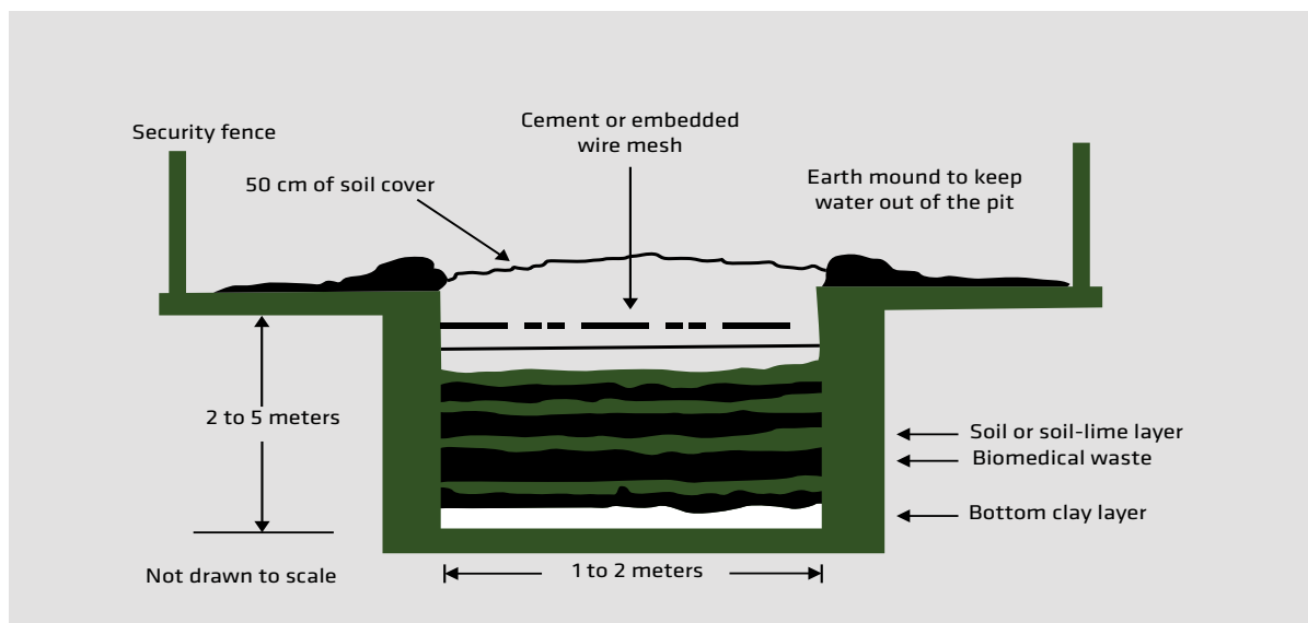
Figure: Layout Specifications for Burial Pit
